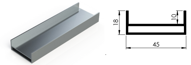
PERFIL U FIJO PA U PROFILE PA FIX PA SYSTEM
