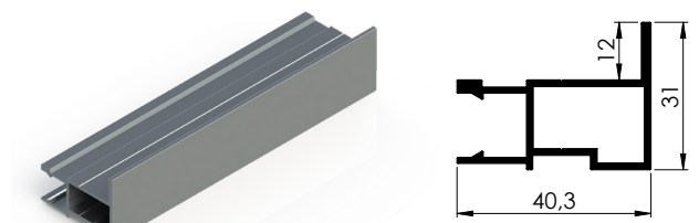
PERFIL BASE FIJO PA BASE PROFILE FIX PA SYSTEM
